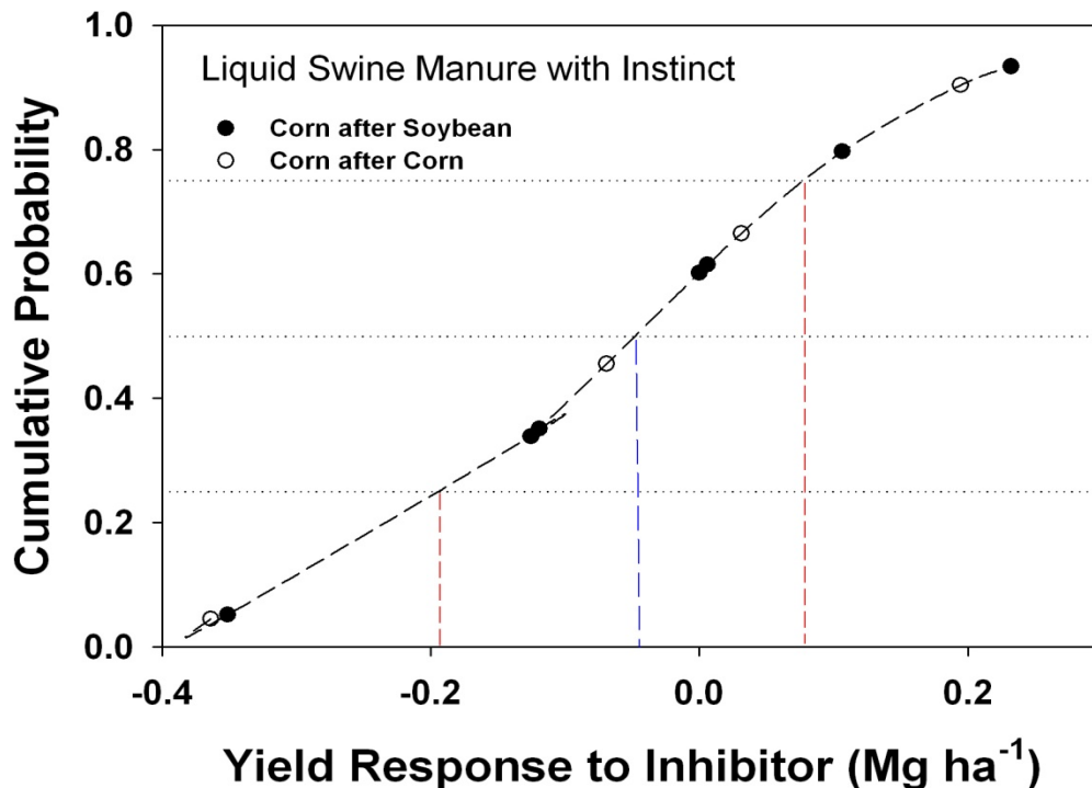
Figure 3. Cumulative probability distribution of yield responses observed by using nitrification inhibitor with fall-applied injected liquid swine manure in 2009.
